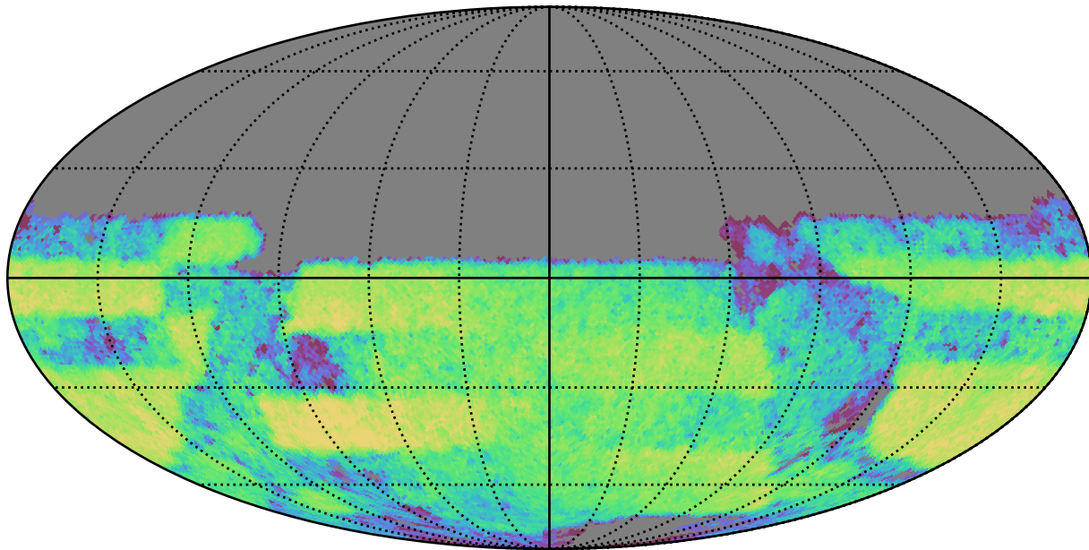
too_10_1v3.4_10yrs Yr 3-4 y band: CoaddM5
