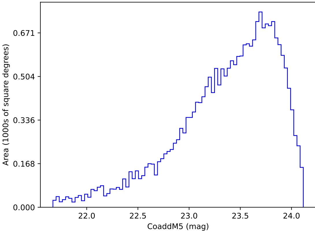
too_10_1v3.4_10yrs Yr 3-4 y band: CoaddM5
