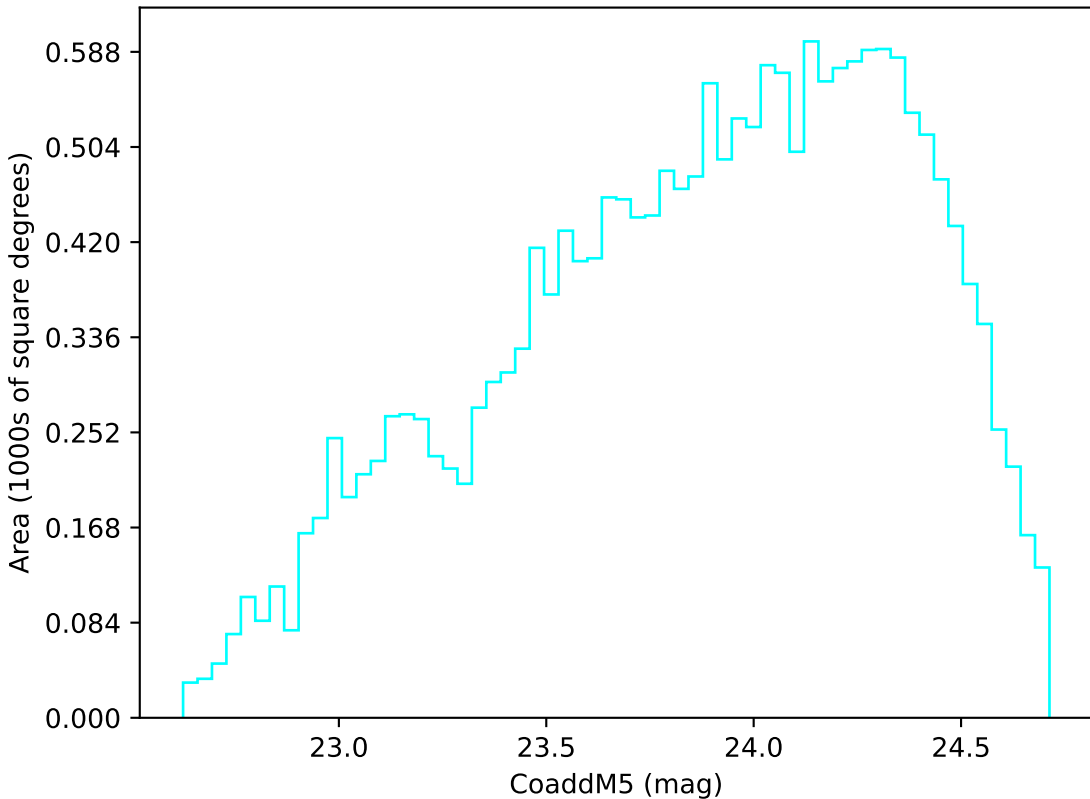
too_10_1v3.4_10yrs Yr 3-4 u band: CoaddM5
