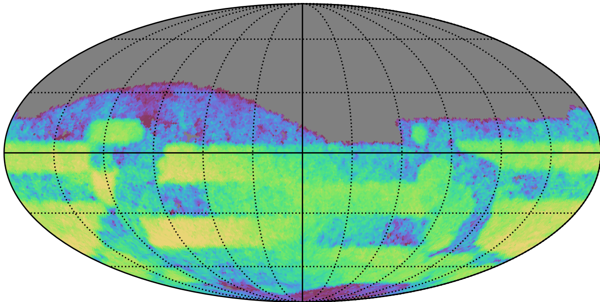
too_10_1v3.4_10yrs Yr 3-4 r band: CoaddM5
