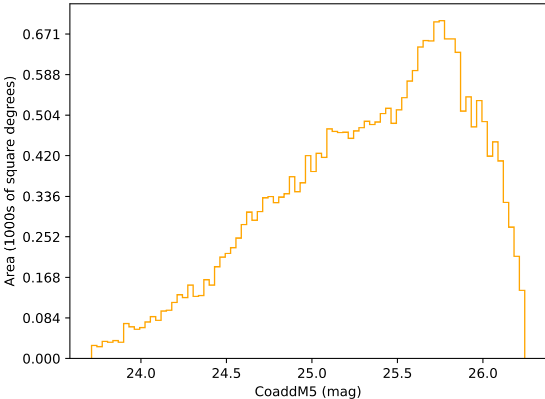
too_10_1v3.4_10yrs Yr 3-4 r band: CoaddM5
