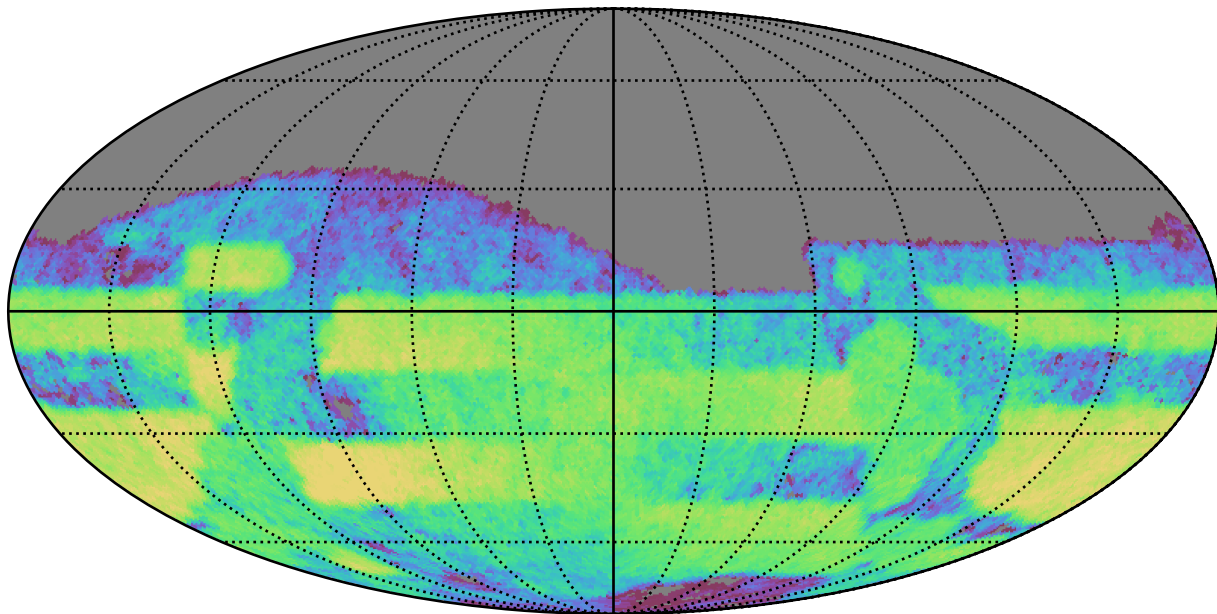
too_10_1v3.4_10yrs Yr 3-4 i band: CoaddM5
