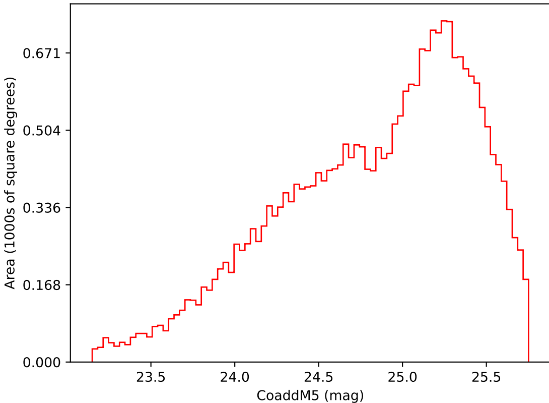
too_10_1v3.4_10yrs Yr 3-4 i band: CoaddM5
