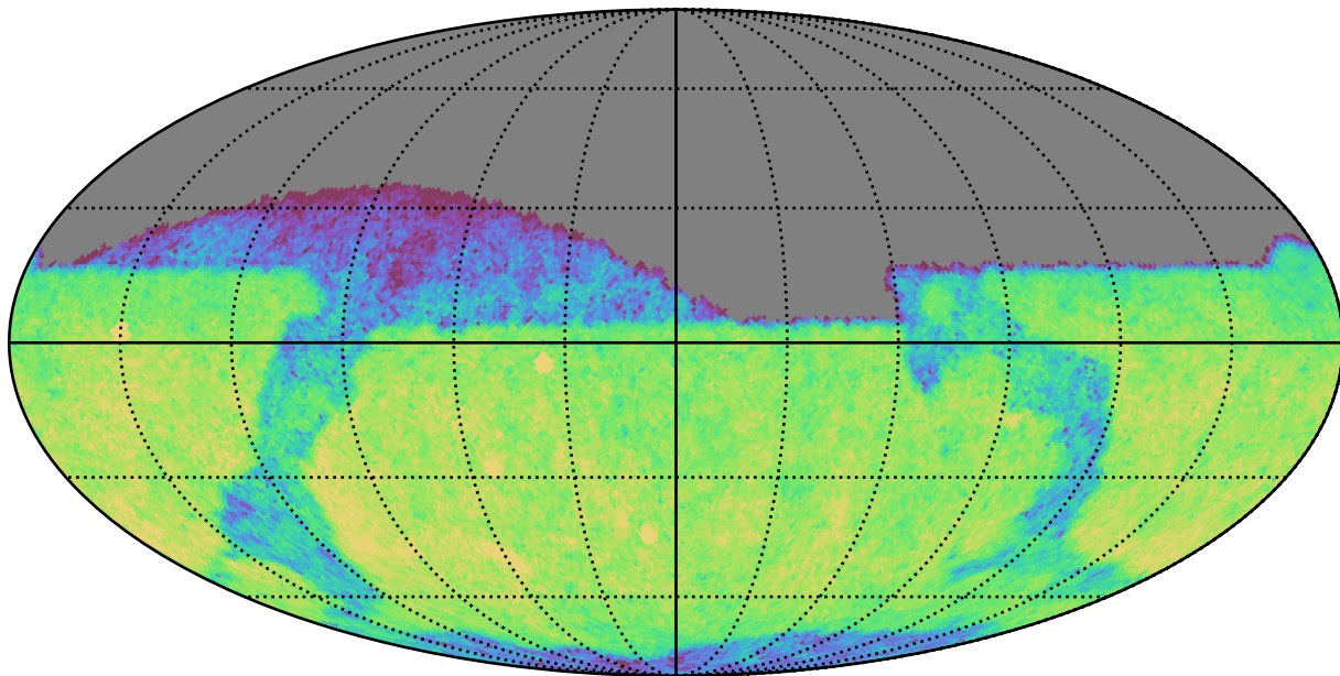
too_10_1v3.4_10yrs Yr 1 z band: CoaddM5
