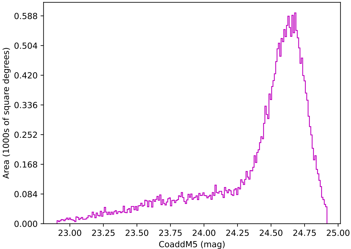
too_10_1v3.4_10yrs Yr 1 z band: CoaddM5
