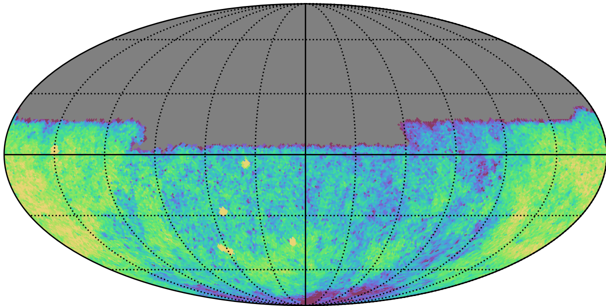
too_10_1v3.4_10yrs Yr 1 u band: CoaddM5
