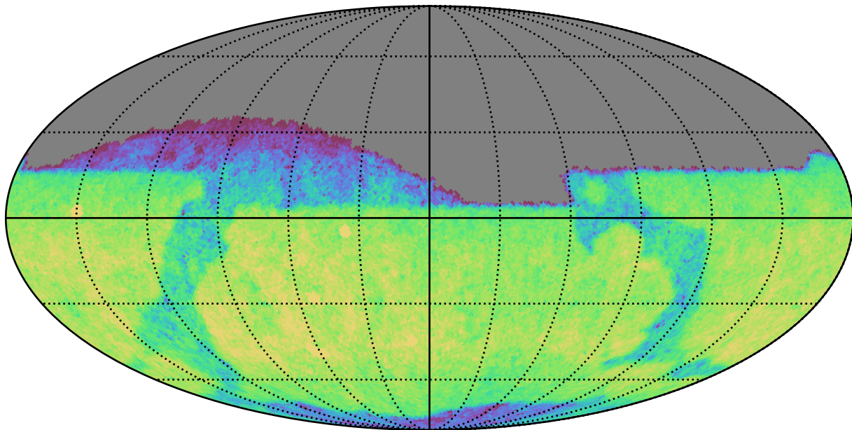
too_10_1v3.4_10yrs Yr 1 r band: CoaddM5
