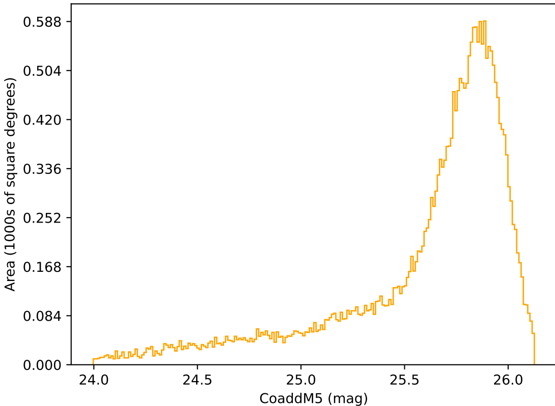
too_10_1v3.4_10yrs Yr 1 r band: CoaddM5
