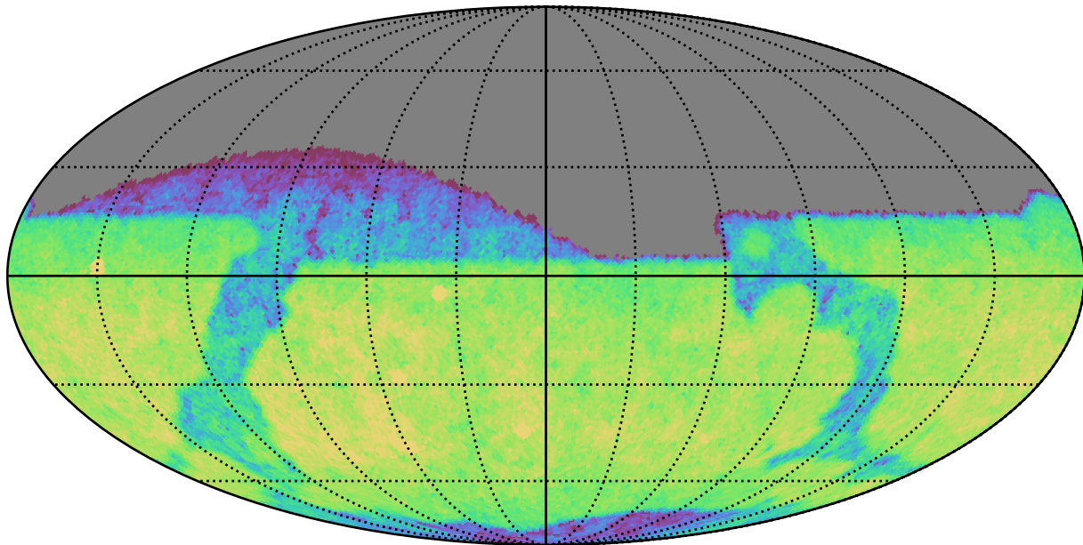
too_10_1v3.4_10yrs Yr 1 i band: CoaddM5
