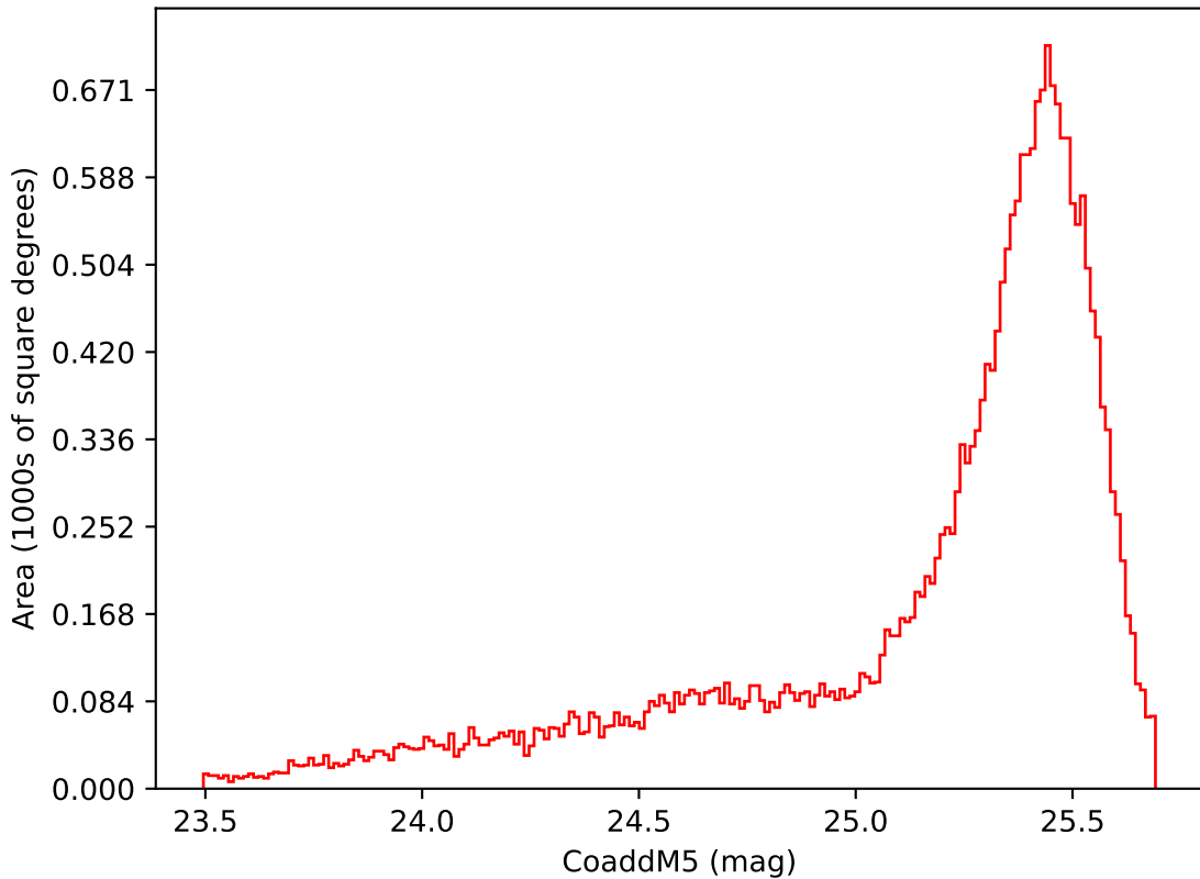
too_10_1v3.4_10yrs Yr 1 i band: CoaddM5
