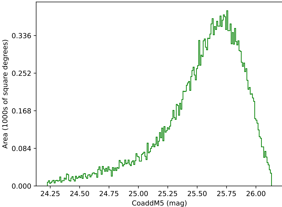
too_10_1v3.4_10yrs Yr 1 g band: CoaddM5
