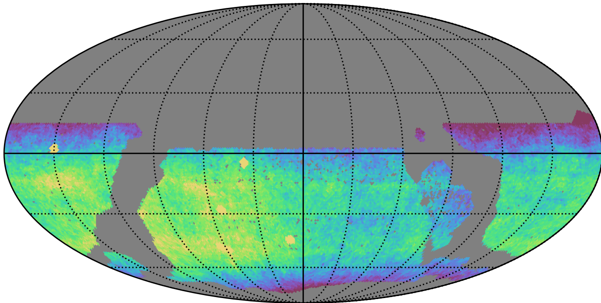
too_10_1v3.4_10yrs WFD z band: CoaddM5
