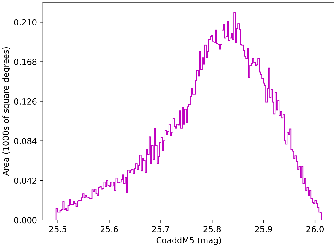
too_10_1v3.4_10yrs WFD z band: CoaddM5
