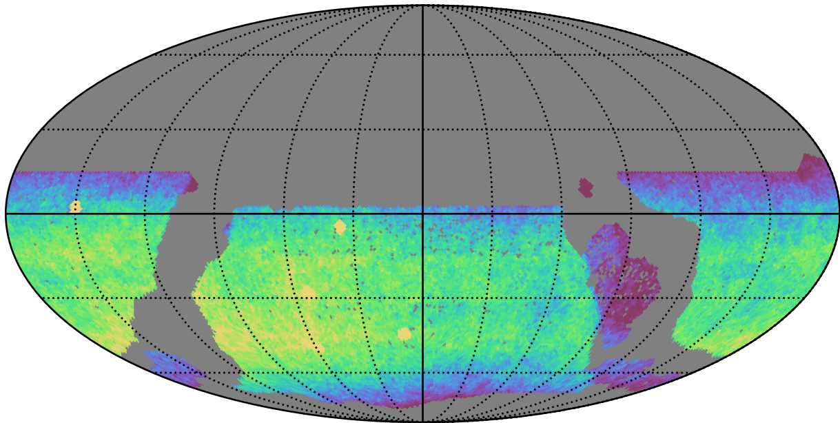
too_10_1v3.4_10yrs WFD y band: CoaddM5
