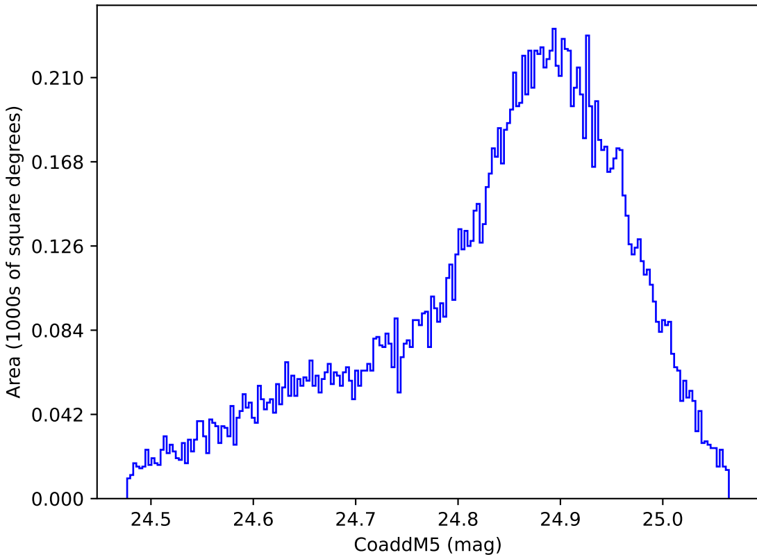
too_10_1v3.4_10yrs WFD y band: CoaddM5
