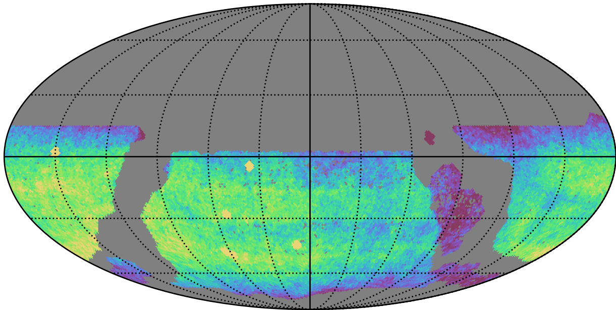
too_10_1v3.4_10yrs WFD u band: CoaddM5
