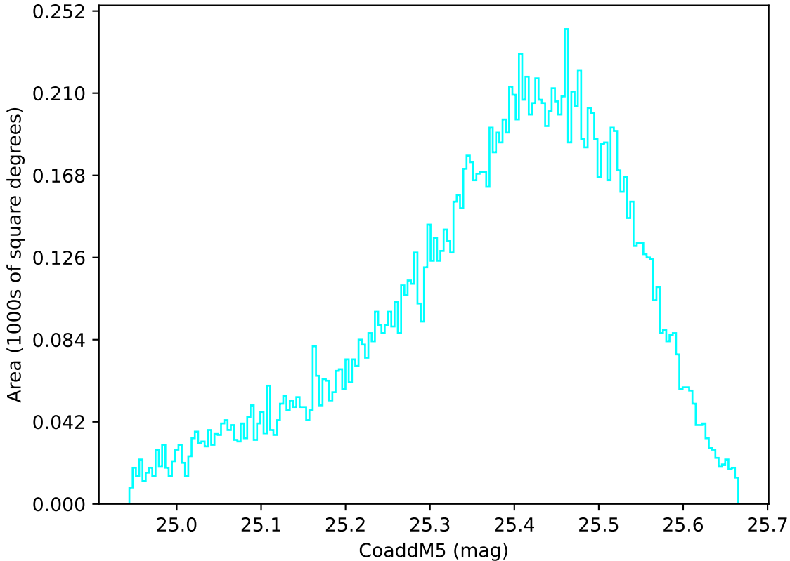
too_10_1v3.4_10yrs WFD u band: CoaddM5
