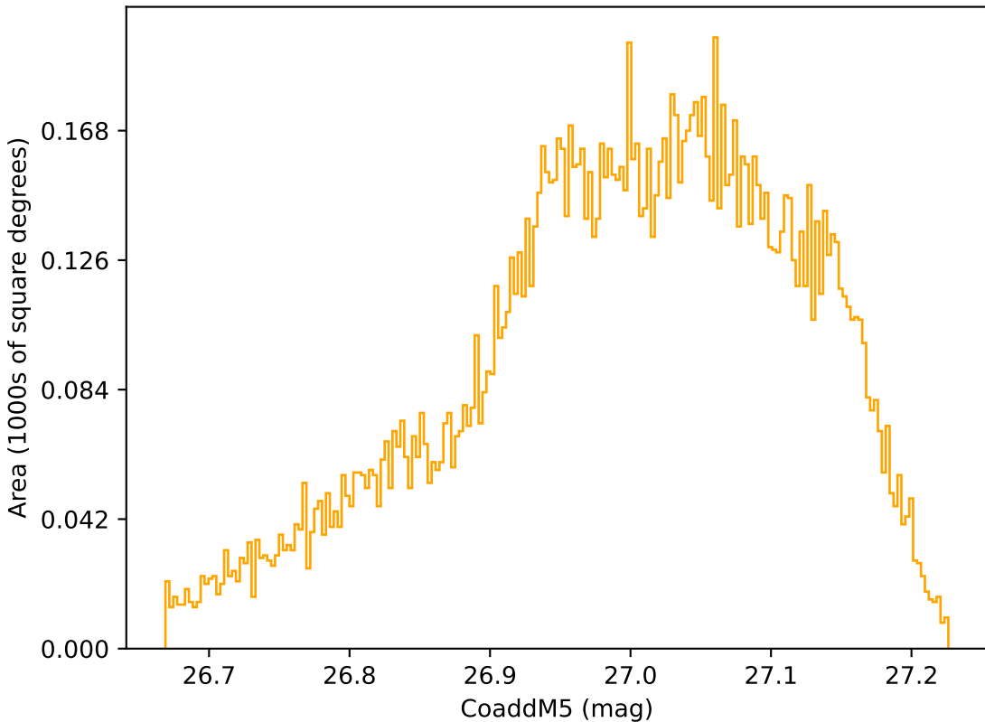
too_10_1v3.4_10yrs WFD r band: CoaddM5
