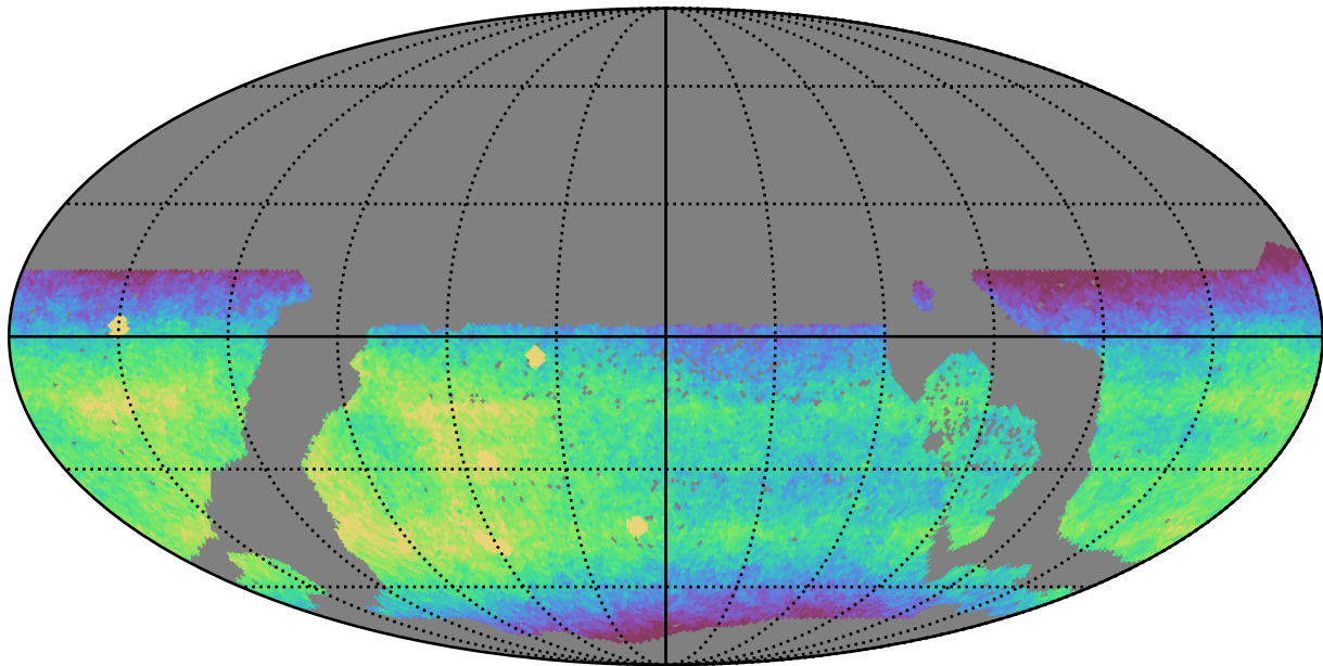
too_10_1v3.4_10yrs WFD i band: CoaddM5
