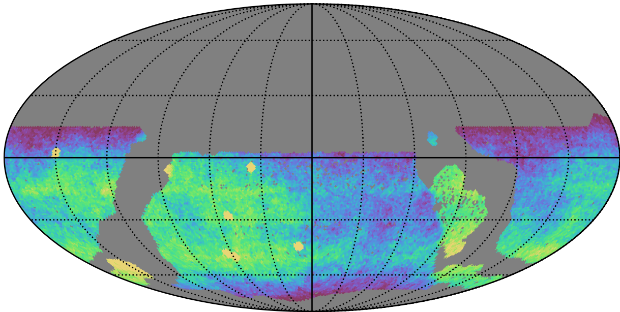
too_10_1v3.4_10yrs WFD g band: CoaddM5
