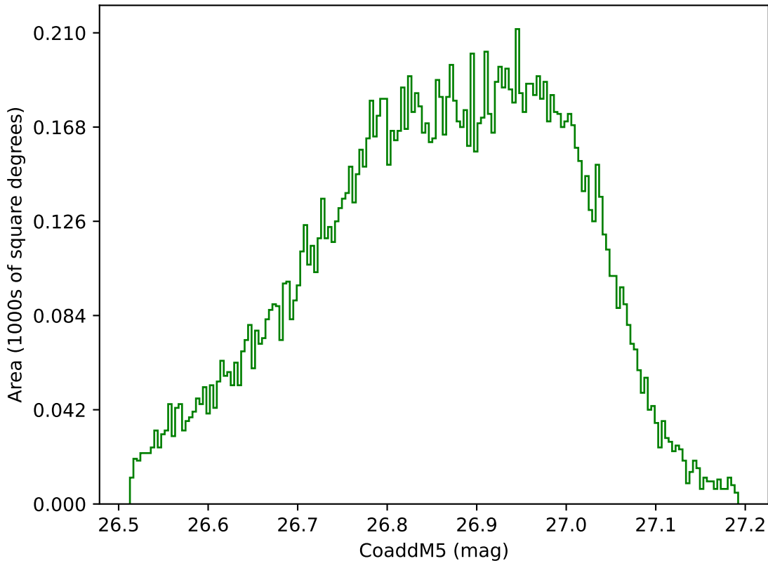
too_10_1v3.4_10yrs WFD g band: CoaddM5
