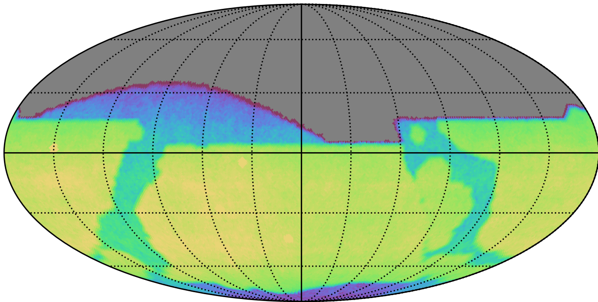
too_10_1v3.4_10yrs All sky z band: CoaddM5
