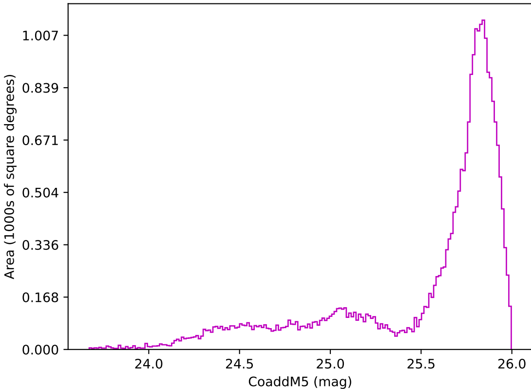
too_10_1v3.4_10yrs All sky z band: CoaddM5
