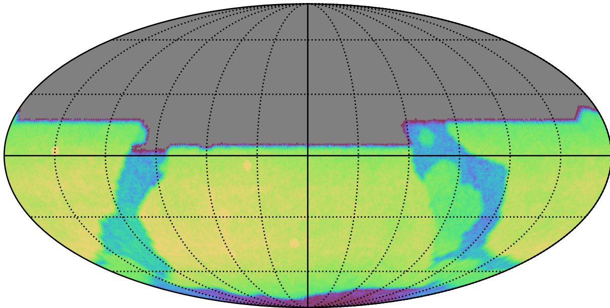
too_10_1v3.4_10yrs All sky y band: CoaddM5
