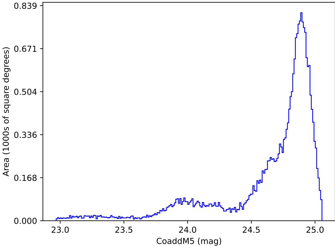
too_10_1v3.4_10yrs All sky y band: CoaddM5
