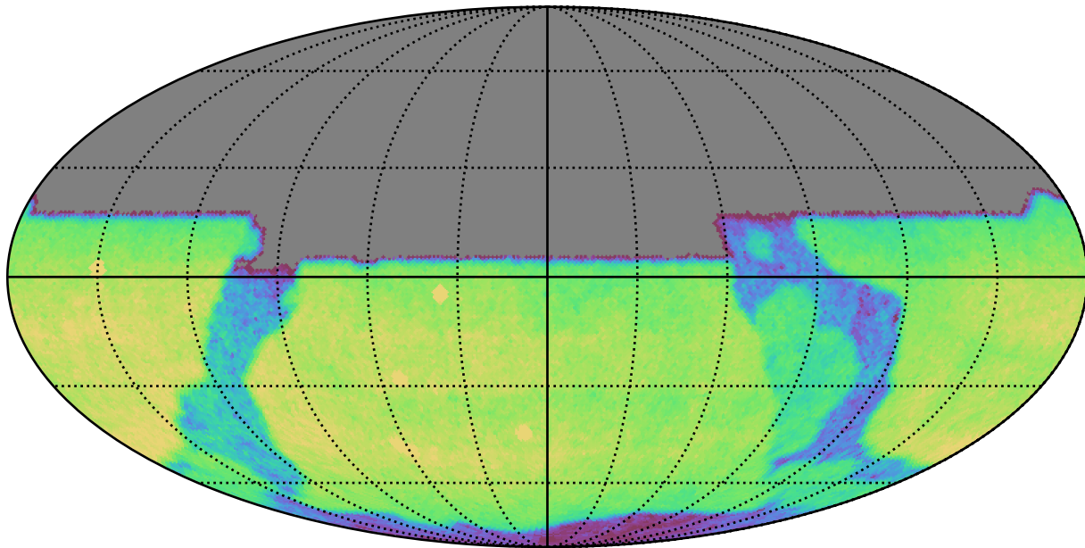
too_10_1v3.4_10yrs All sky u band: CoaddM5
