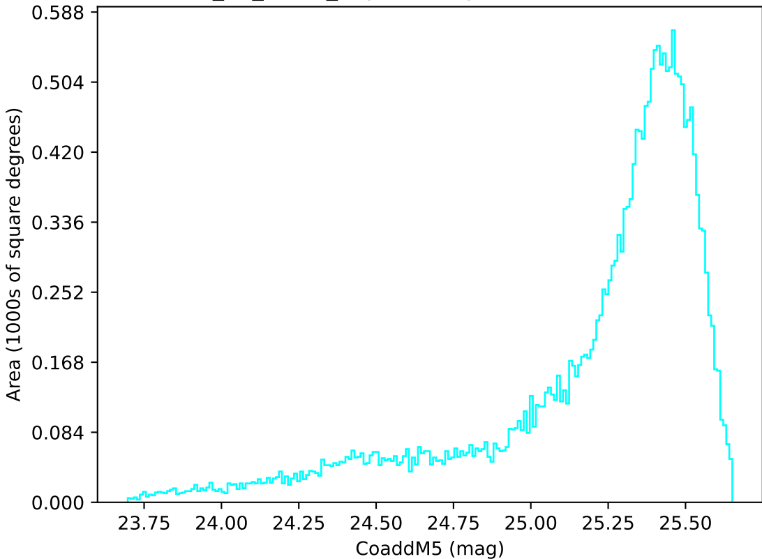
too_10_1v3.4_10yrs All sky u band: CoaddM5
