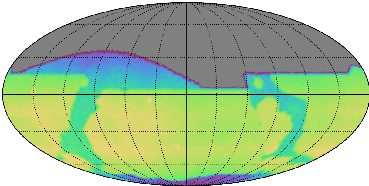
too_10_1v3.4_10yrs All sky r band: CoaddM5
