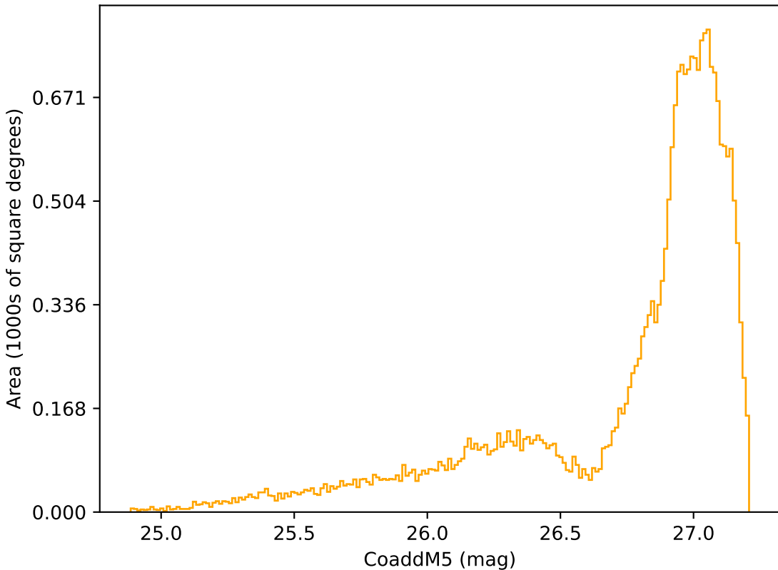
too_10_1v3.4_10yrs All sky r band: CoaddM5
