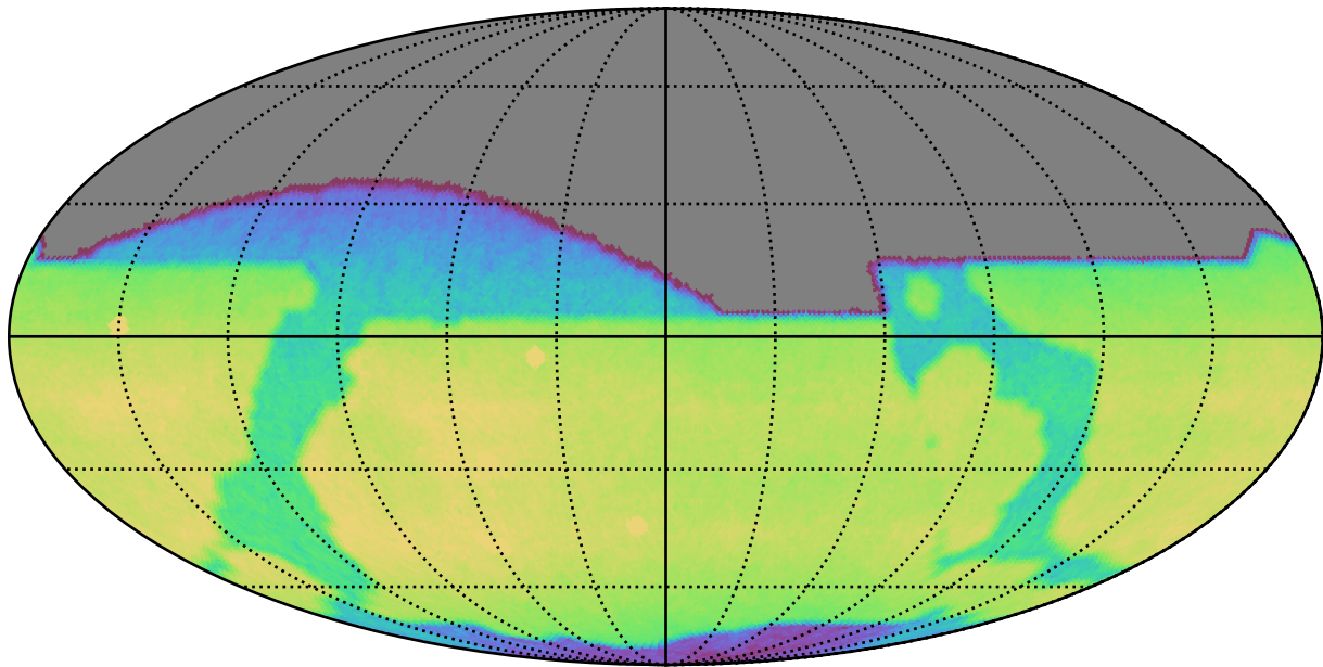
too_10_1v3.4_10yrs All sky i band: CoaddM5
