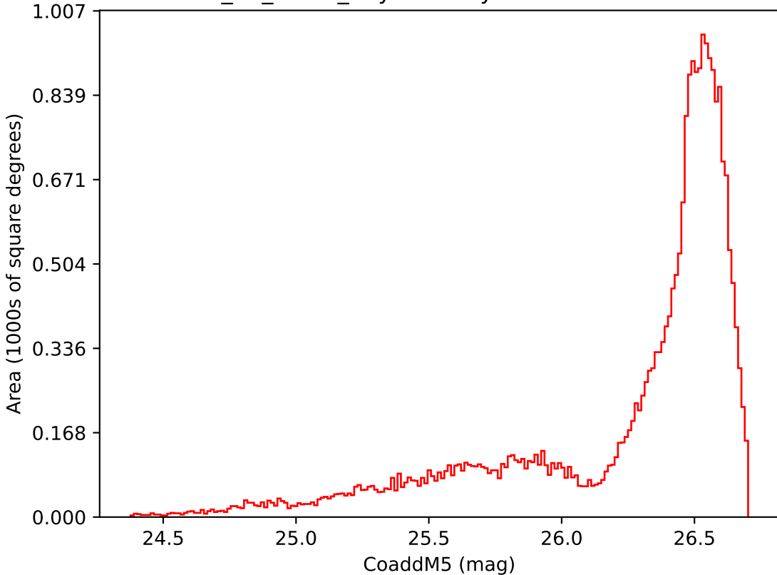
too_10_1v3.4_10yrs All sky i band: CoaddM5
