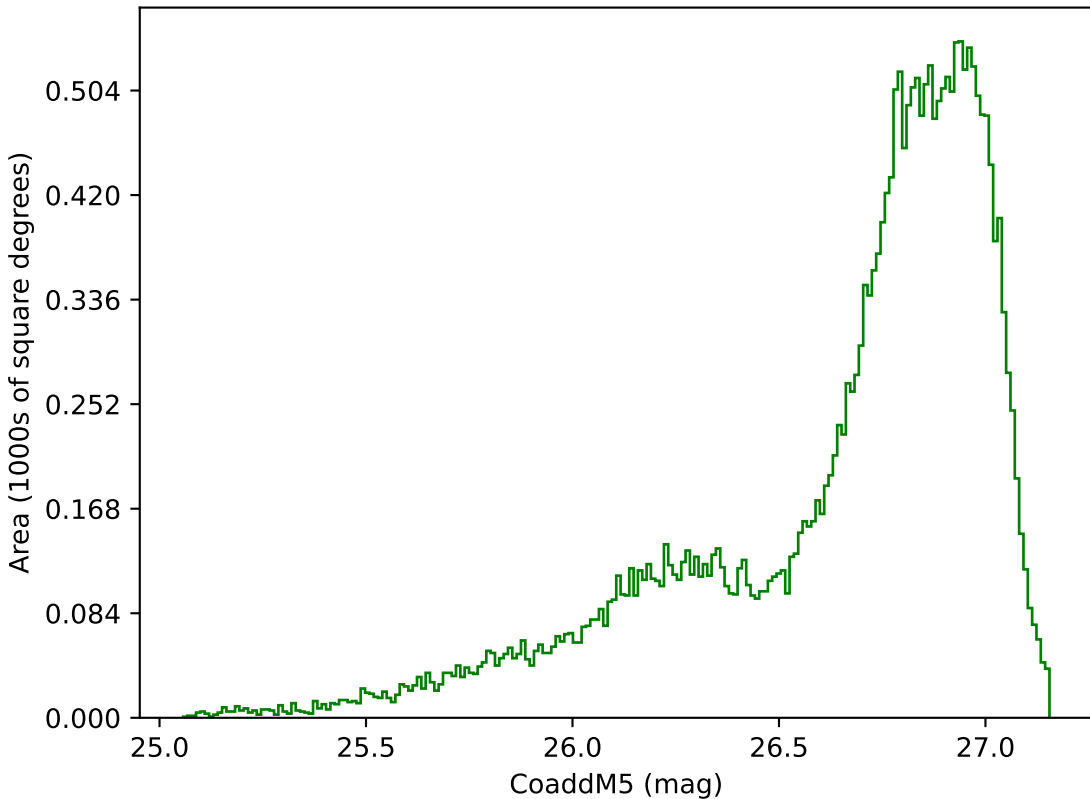
too_10_1v3.4_10yrs All sky g band: CoaddM5
