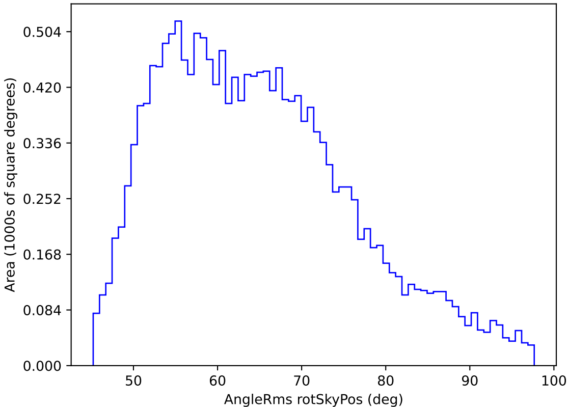
too_10_1v3.4_10yrs WFD u band: AngleRms rotSkyPos
