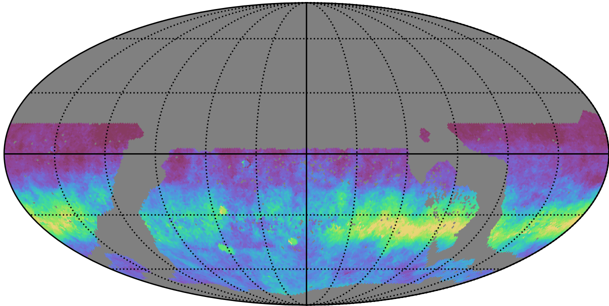
too_10_1v3.4_10yrs WFD r band: AngleRms rotSkyPos
