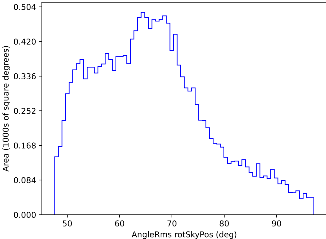
too_10_1v3.4_10yrs WFD r band: AngleRms rotSkyPos
