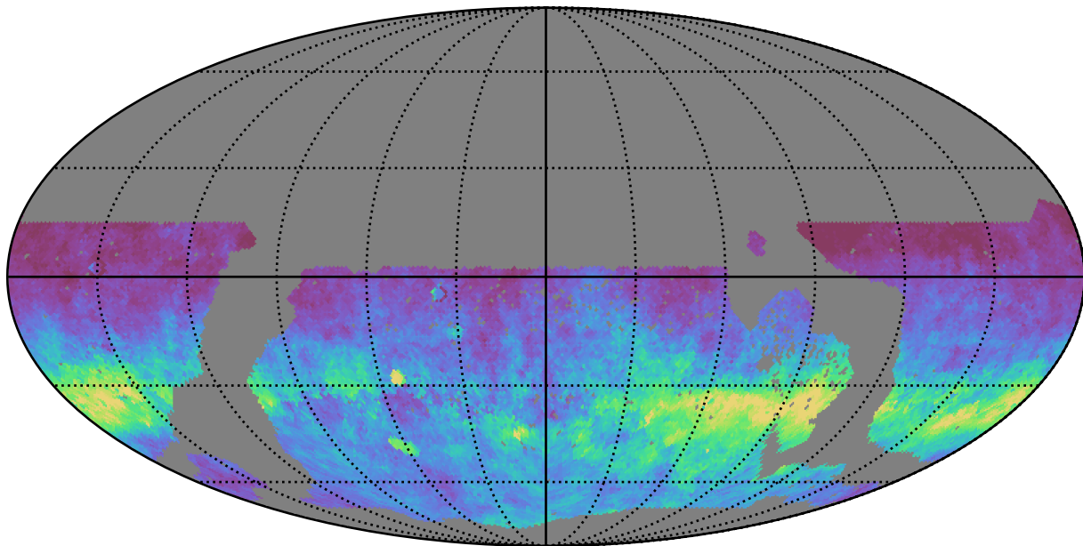
too_10_1v3.4_10yrs WFD i band: AngleRms rotSkyPos
