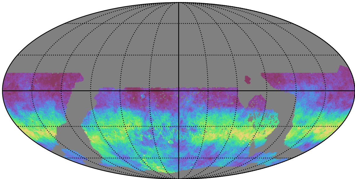
too_10_1v3.4_10yrs WFD g band: AngleRms rotSkyPos
