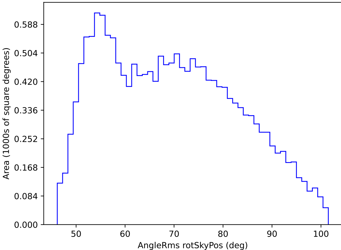
too_10_1v3.4_10yrs WFD g band: AngleRms rotSkyPos
