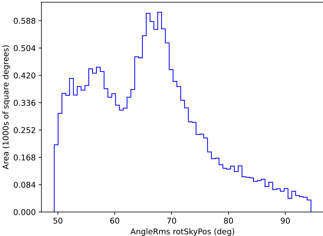
too_10_1v3.4_10yrs WFD all bands: AngleRms rotSkyPos
