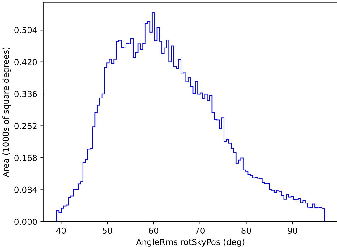
too_10_1v3.4_10yrs All sky z band: AngleRms rotSkyPos
