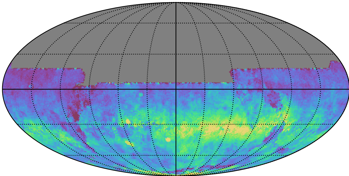
too_10_1v3.4_10yrs All sky y band: AngleRms rotSkyPos
