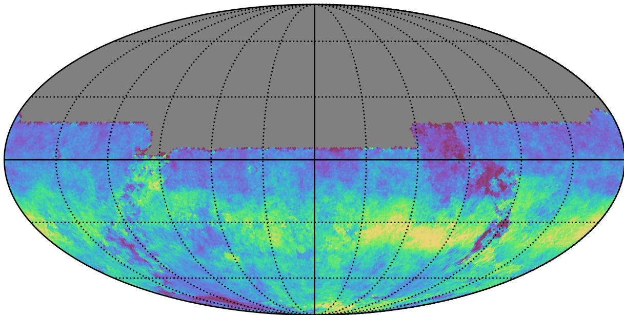
too_10_1v3.4_10yrs All sky u band: AngleRms rotSkyPos
