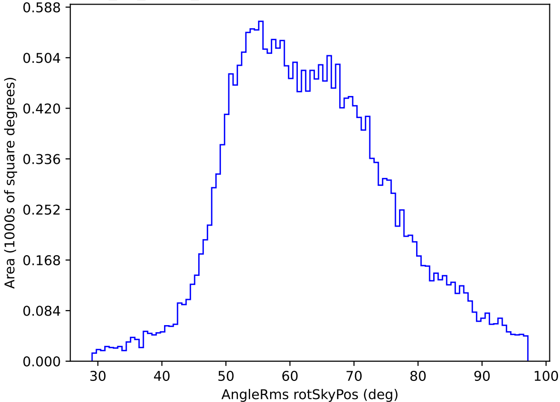
too_10_1v3.4_10yrs All sky u band: AngleRms rotSkyPos
