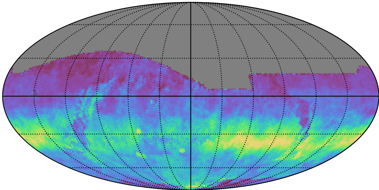
too_10_1v3.4_10yrs All sky r band: AngleRms rotSkyPos
