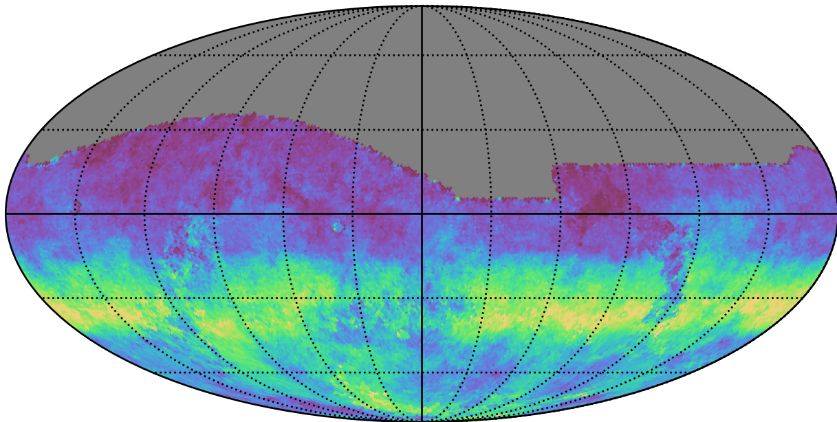
too_10_1v3.4_10yrs All sky g band: AngleRms rotSkyPos
