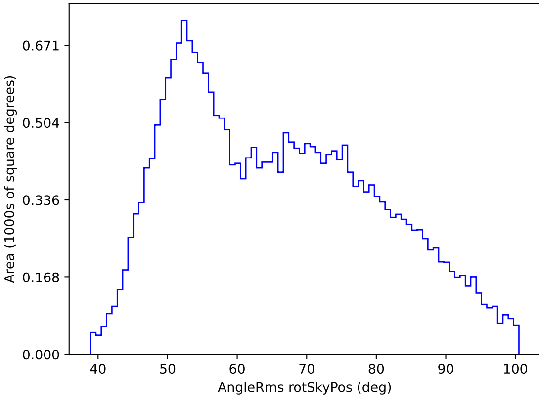
too_10_1v3.4_10yrs All sky g band: AngleRms rotSkyPos
